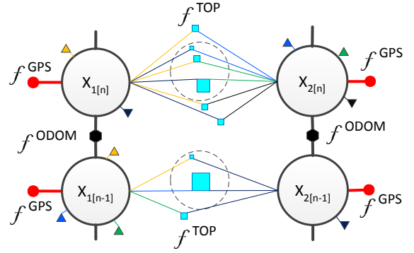
Fig. 3. Factor graph for (n-1) and n^{\text{th}} state of two vehicles with four state nodes, two Odometry factors, four GPS factors and nine topology factors. Dotted circle represents Gate Boundary for PDA Filter. Triangles represent the RADAR readings of the vehicles associated with the states.
