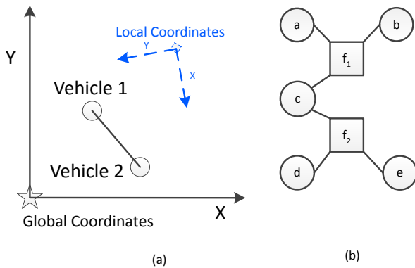
Fig. 1. (a) Topology for vehicle infrastructure CL. Dashed Axis in blue represent the coordinate system of the RADAR. (b) Factor graph with variables a, b, c, d, e and functions f_1(a, b, c) and f_2(c, d, e) .
