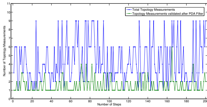
Fig. 7. Comparison of validated measurements by PDA Filter and the total measurements for Fig. 4(a) (refer Results).
