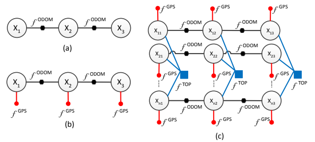
Fig. 2. (a) Factor graph with three state nodes and two odometry factors. (b) Factor graph with three state nodes, two odometry factors and three GPS factors. (c) Factor graph for n vehicles with three state nodes, two odometry factors, three GPS factors and two topology factors each.
